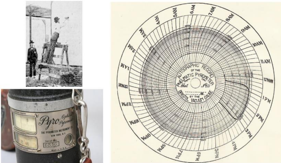
Figure 7. Pyrometer Temperature Recorded Measurement (see [27]).
