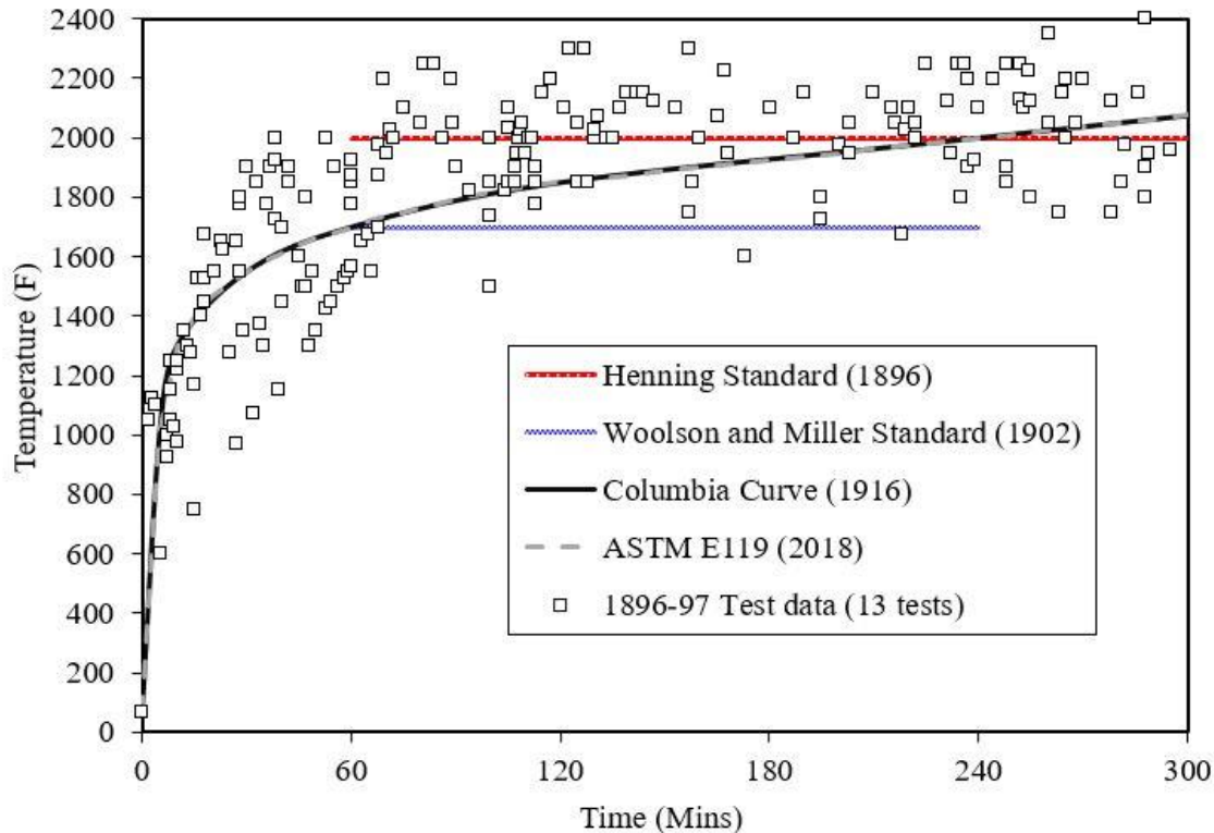
Figure 8. Author's subjective Evolution of Fire Time-Temperature Curves as adopted by ASTM [39].
